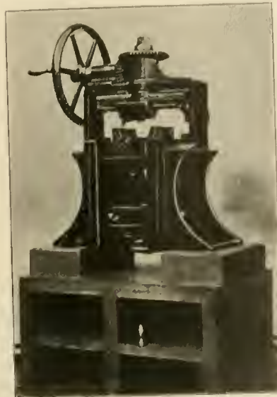
ROTARY PLANER FOR ROD BRASSES.
